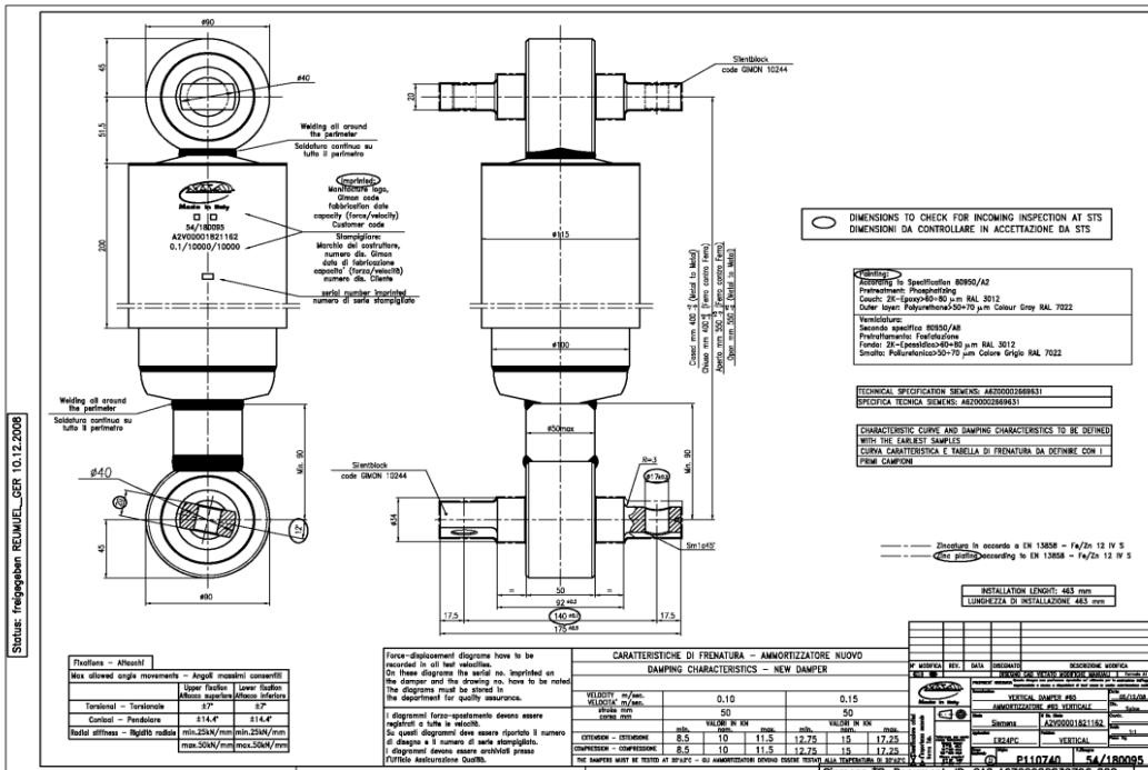
DAMPER SECONDARY VERTICAL (A2V00001821162)
